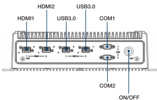
Front Panel
