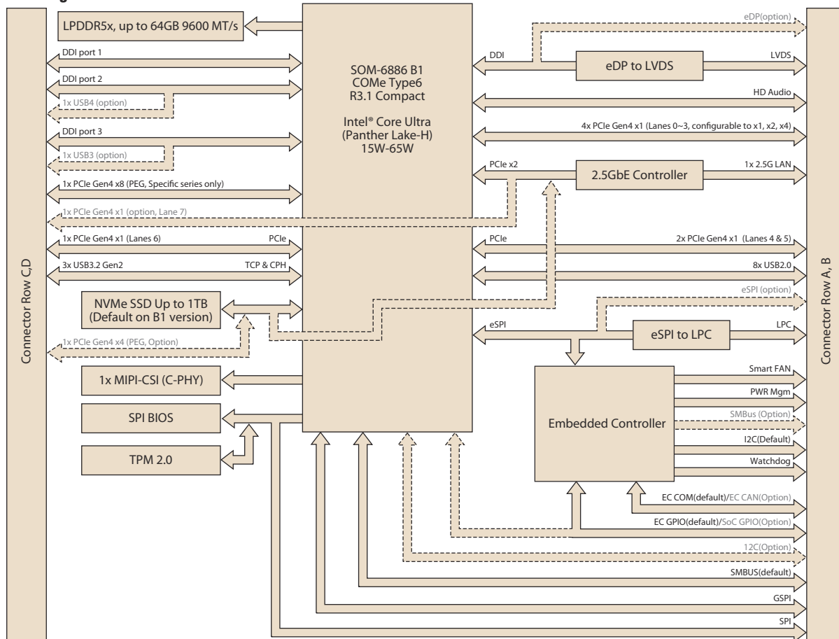
Block Diagram for B1
