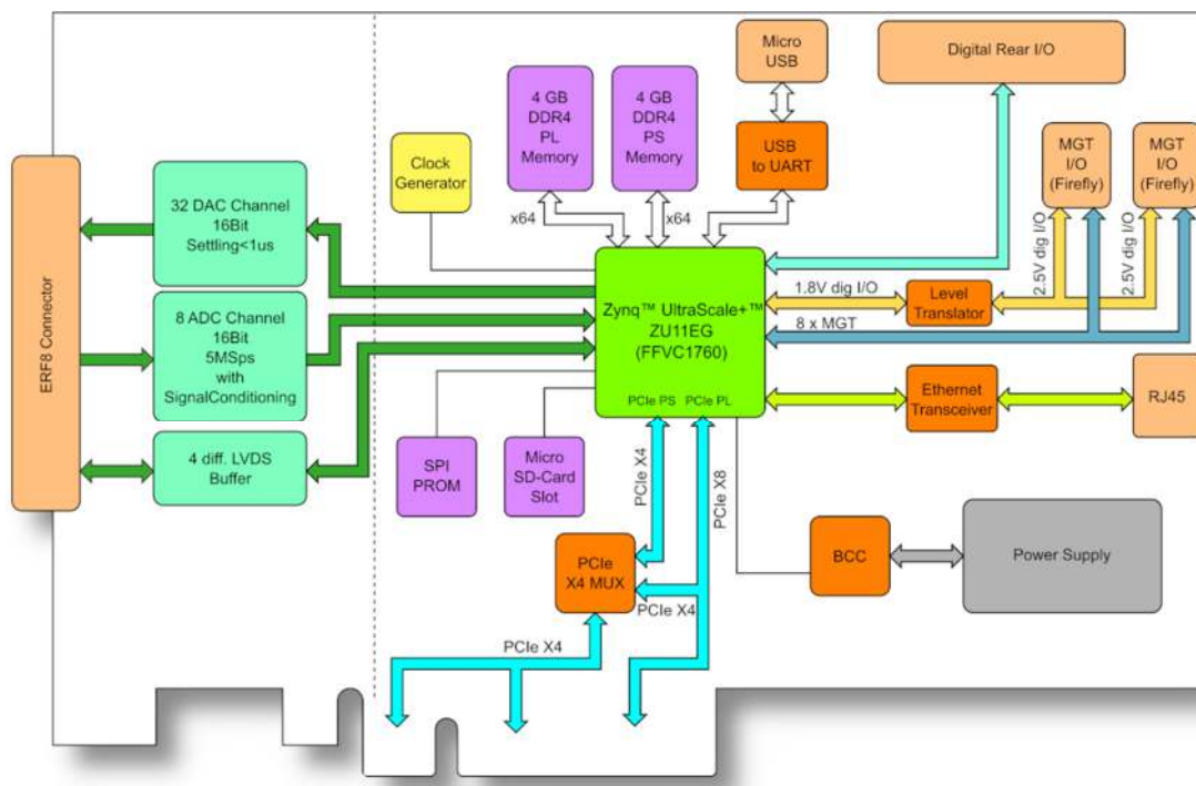
Block Diagram TPCE646
