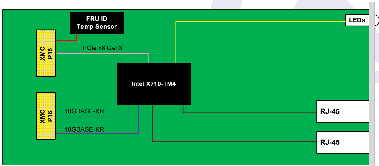
Figure 2: Functional block diagram (Dual 10GBASE-T front I/O and Dual 10GBASE-KR rear I/O)
